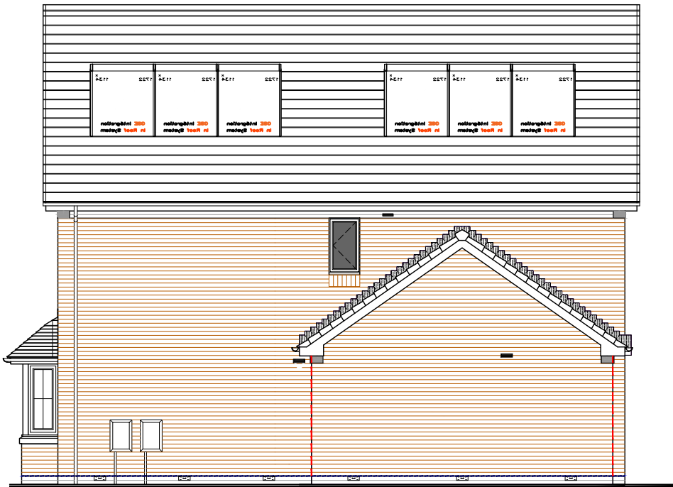
FRONT ELEVATION
